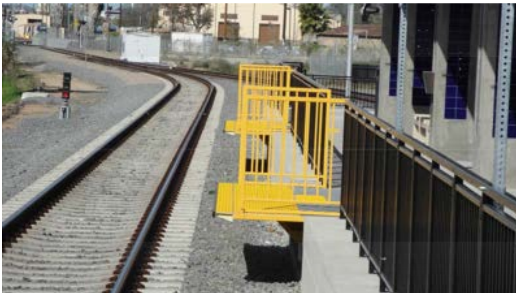
Figure 26. Station-based Retractable (Flip-up) Platform Edges Source: North County Transit District, 2010
